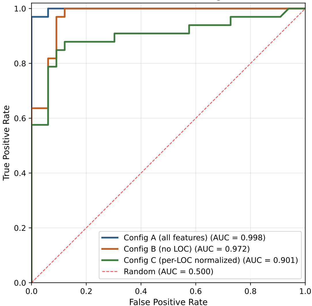
ROC curves across three configurations
